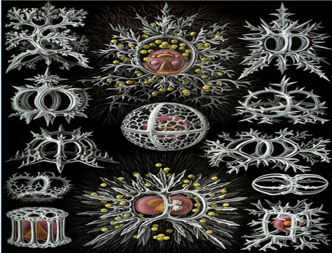
Haeckel's Radiolarians
